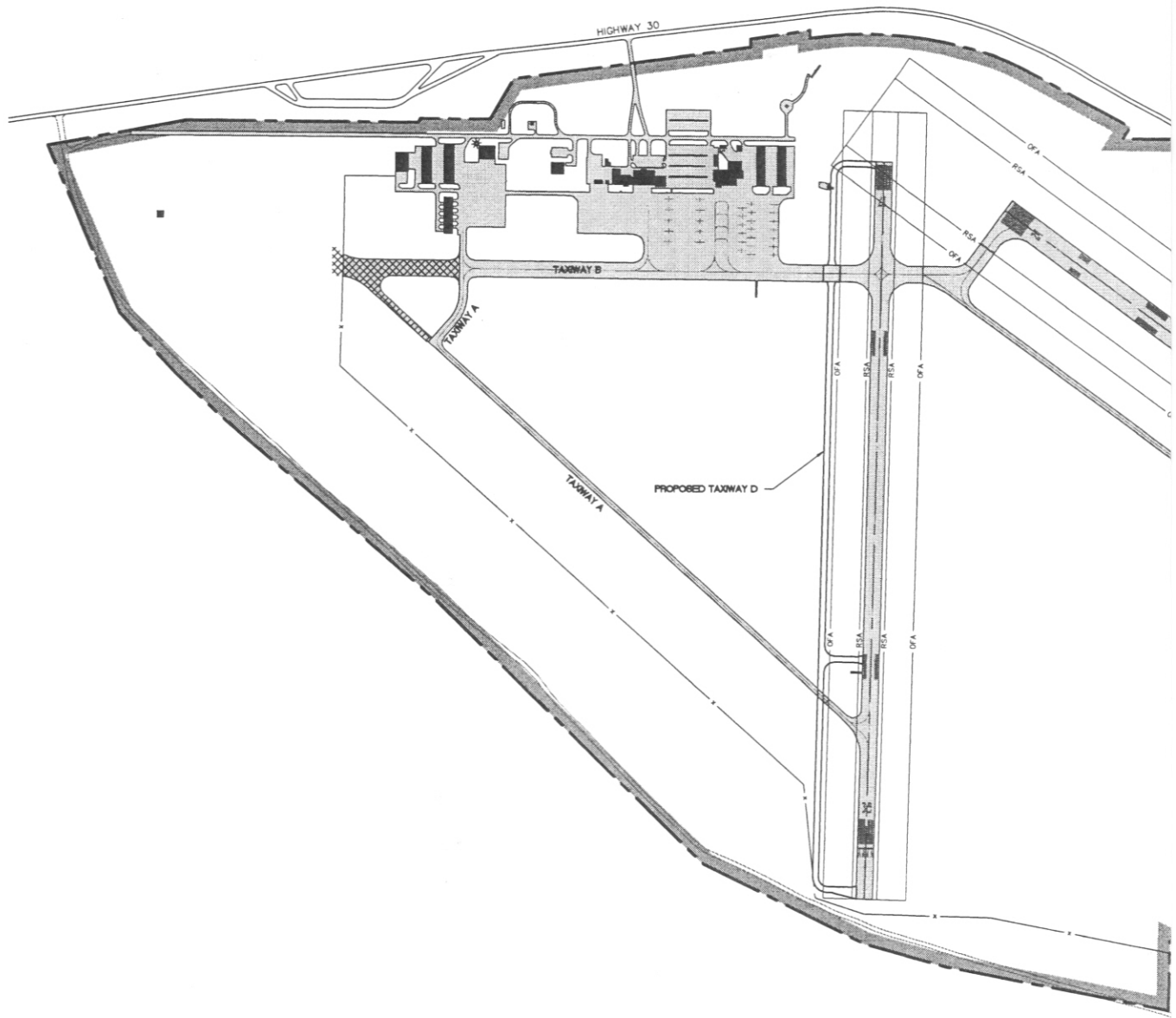
PROJECT LAYOUT PLAN SCALE: 1" = 500'
